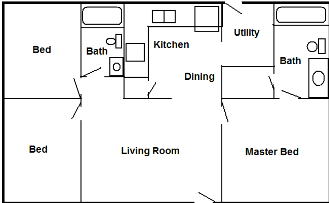
Floor Plan
